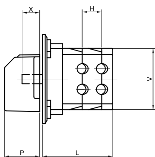
S 16, 25, 32, 40 J
