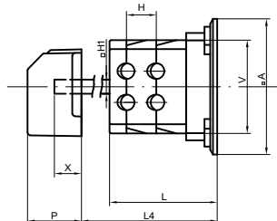
S 16, 25, 32, 40 JO
