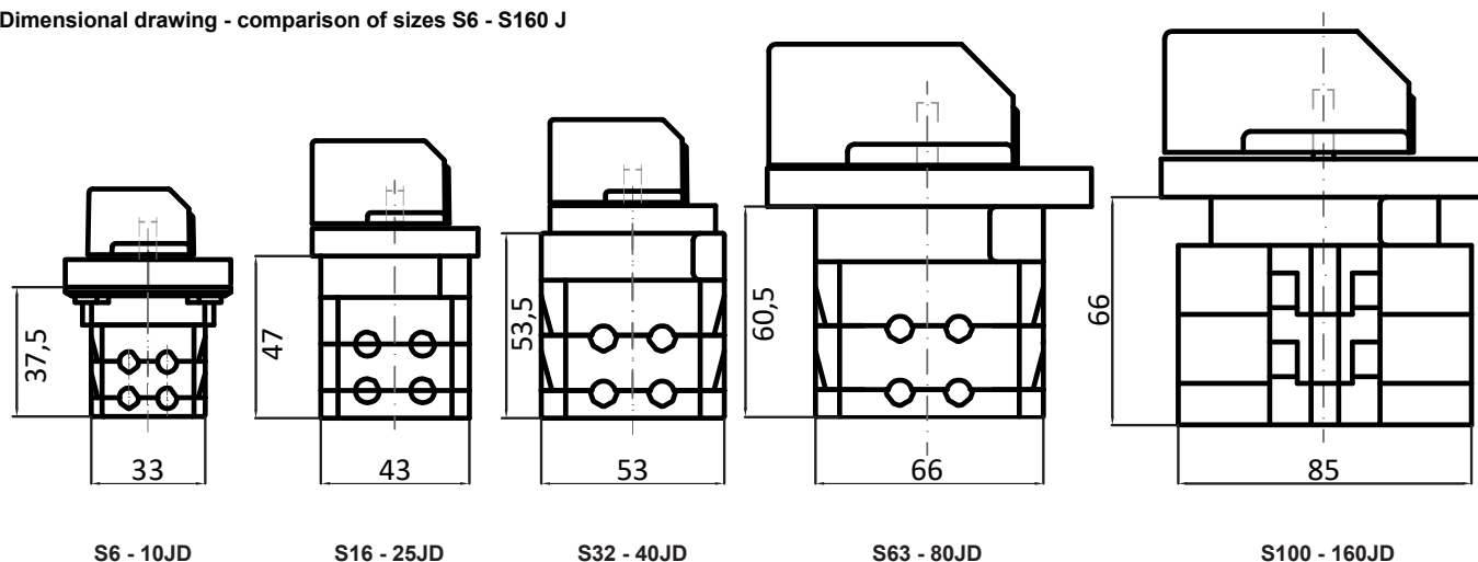
Dimensional drawing - comparison of sizes S6 - S160 J
