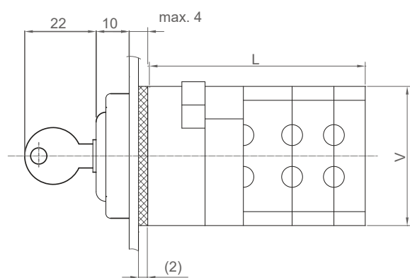
S 16, 25 JKD
