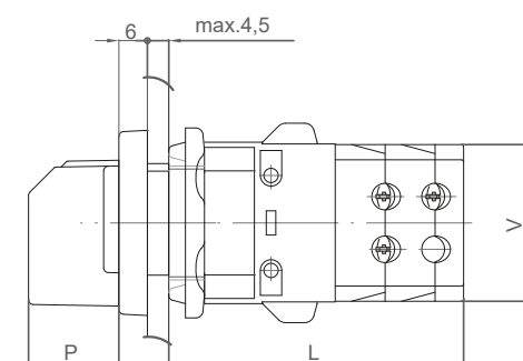
S 6, 10 JRD
