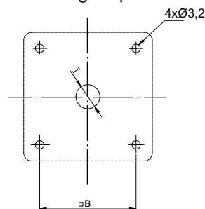
mounting on panel
