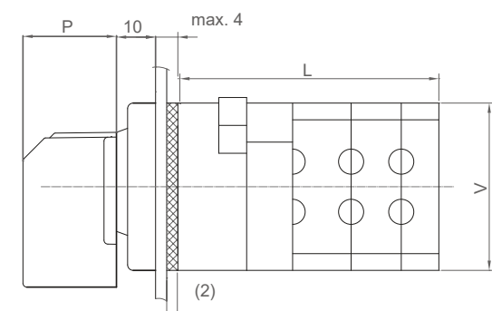
S 16, 25 JRD
