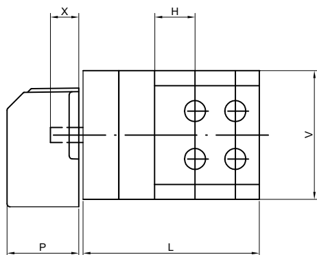
S 16, 25, 32, 40 JV
