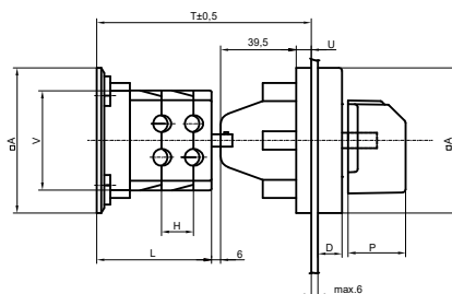
S 16, 25, 32, 40 JBD
