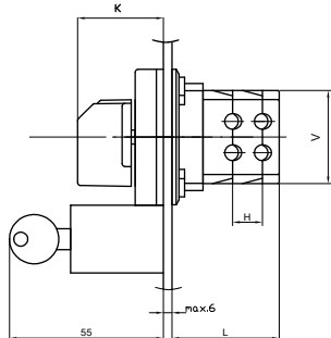
S 16, 25, 32, 40 JZ
