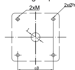
mounting on panel
