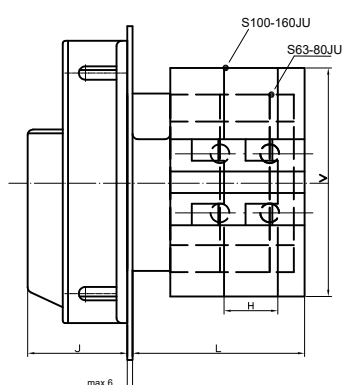
S 63, 80, 100, 125, 160 JU
