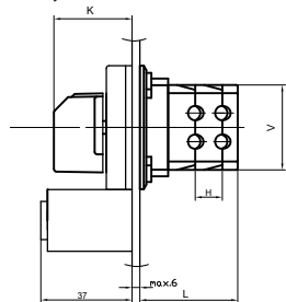
S 16, 25, 32, 40 JT
