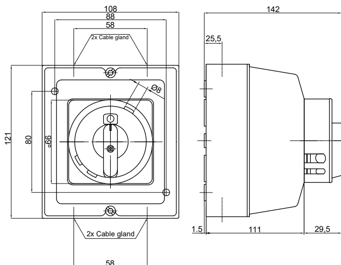
S 32, 40, 63, 80 JNPU
