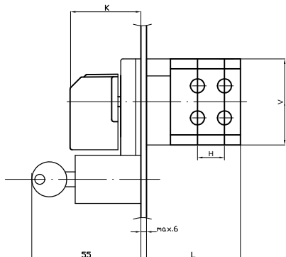
S 63, 80, 100, 125, 160 JZ
