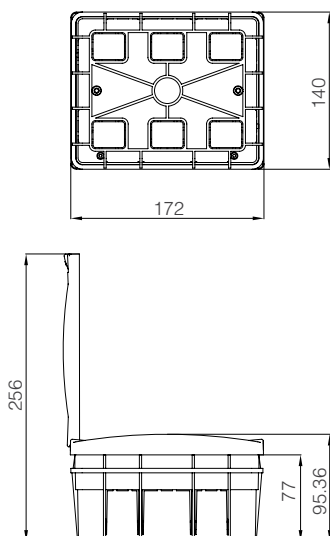
Flush Mount Distribution Box with Terminal Module 6
