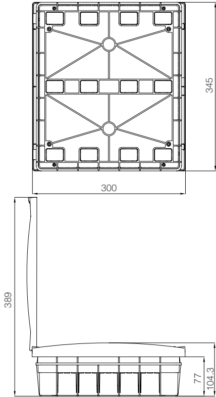
Flush Mount Distribution Box with Terminal Module 24 Double Decker
