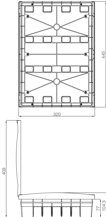
Flush Mount Distribution Box with Terminal Module 36 Threefold
