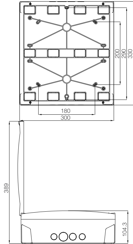
Surface Mount Distribution Box with Terminal Module 24 Double Decker
